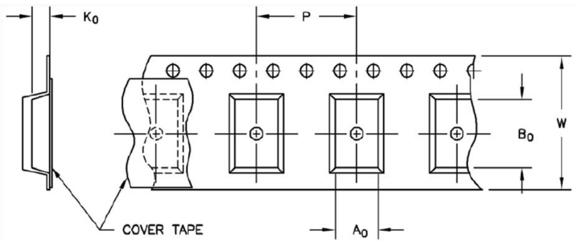
Component Taping Orientation for 28-Lead PLCC Devices
