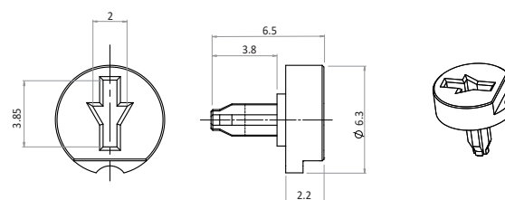
Fig. 6 - Ref.: 6160 For W rotors only.
