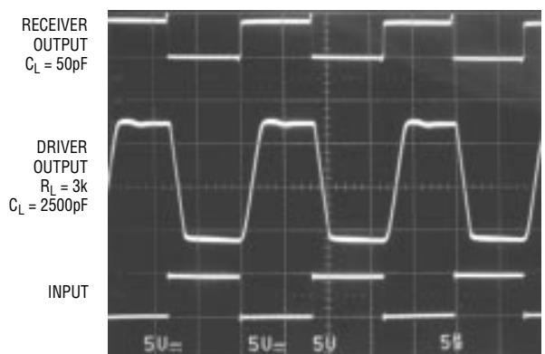
Output Waveforms
