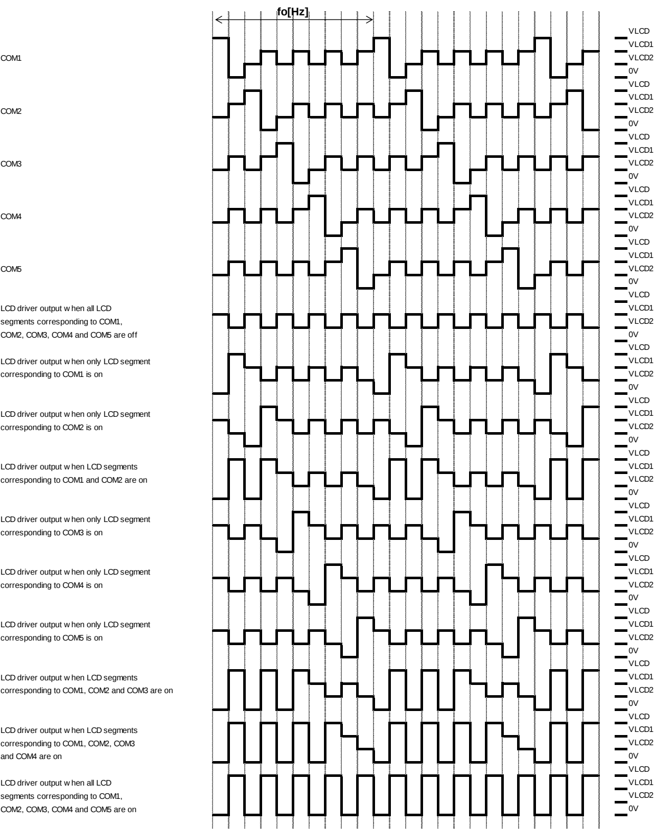
Figure 24. LCD Waveform (Line Inversion, 1/5 Duty, 1/3 Bias)
