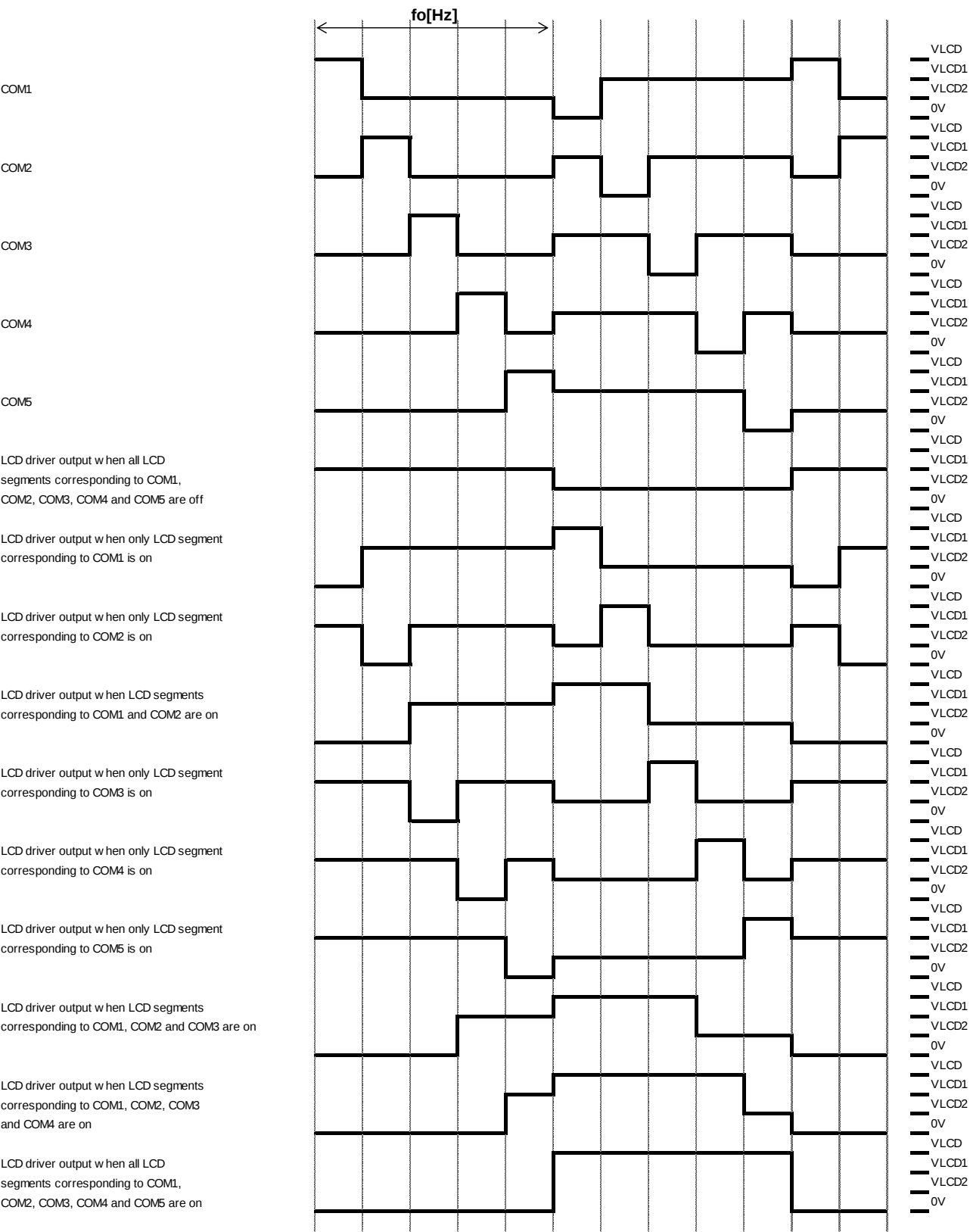
Figure 31. LCD Waveform (Frame Inversion, 1/5 Duty, 1/3Bias)
