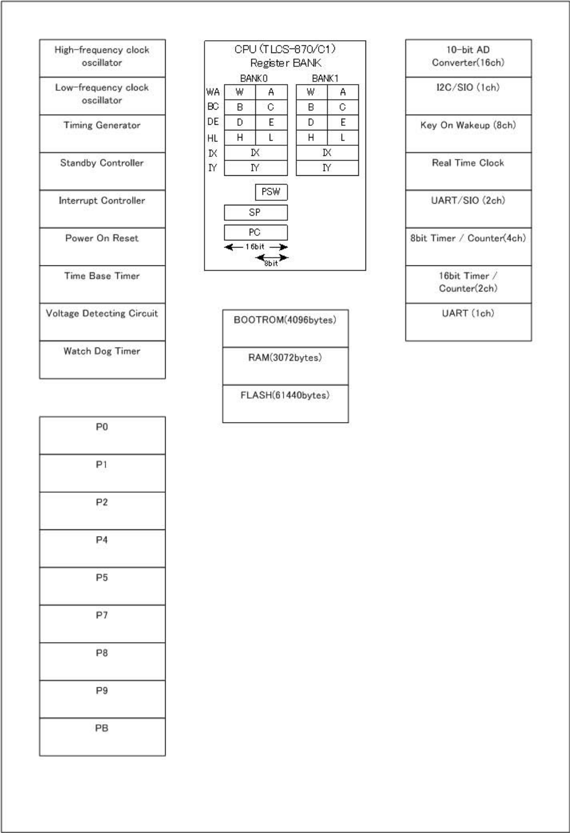
Figure 1-2 Block Diagram
