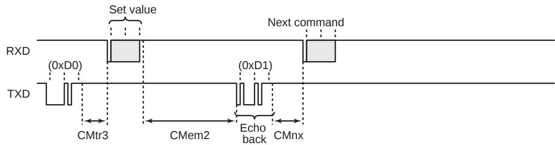
Figure 22-14 Mask ROM Emulation Setting Command
