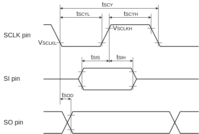
Figure 17-17 AC Characteristics
