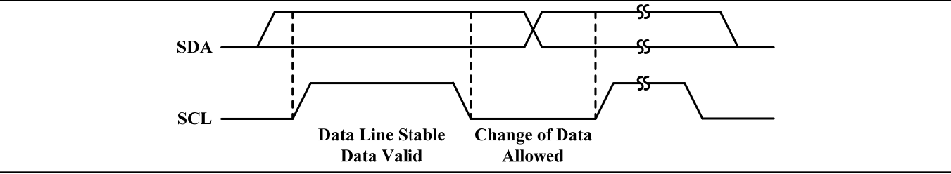
Figure 4 Bit transfer
