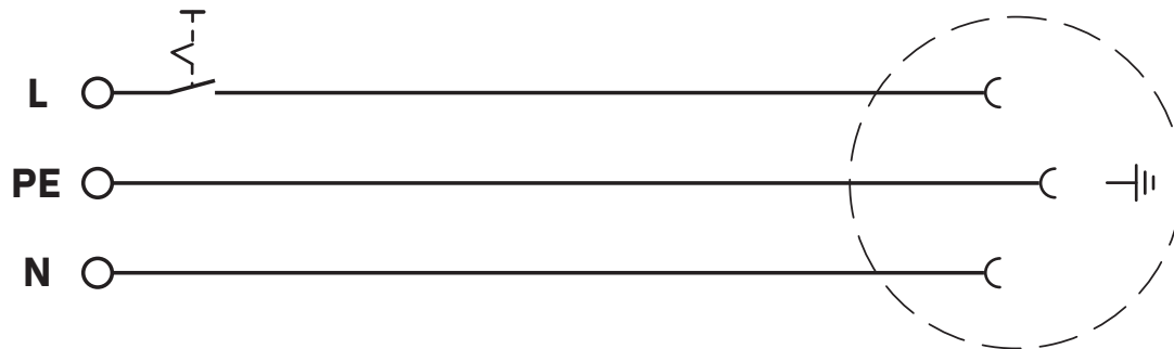
Circuit diagram
