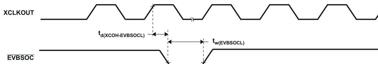
Figure 8-18. EVBSOC Timing
