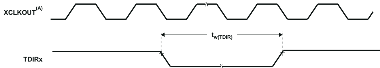
Figure 8-16. TDIRx Timing
