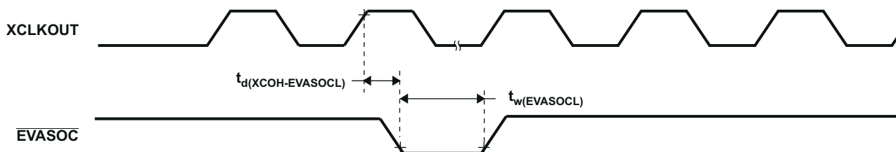
Figure 8-17. EVASOC Timing
