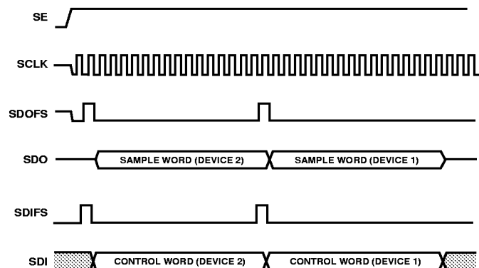
Figure 15. Interface Signal Timing for Control Mode Operation
