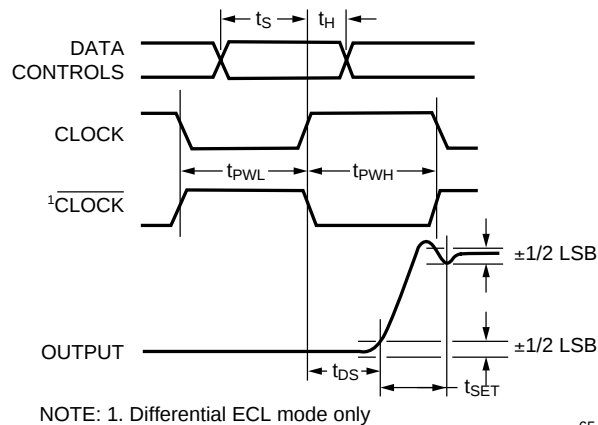
Figure 1. Timing Diagram
