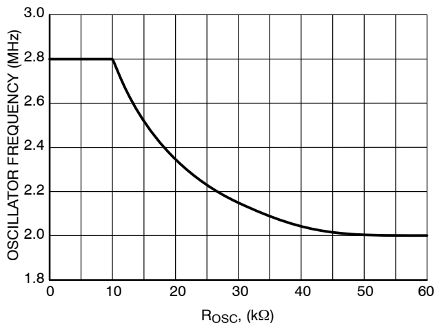
Figure 22. Oscillator Frequency vs. ROSC Value
