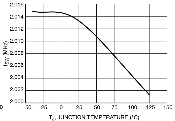
Figure 8. F SW vs. Junction Temperature
