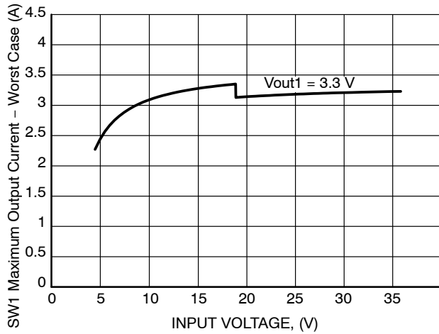
Figure 30. Switcher 1 Load Current Capability with a 4.7 \mu H Inductor
