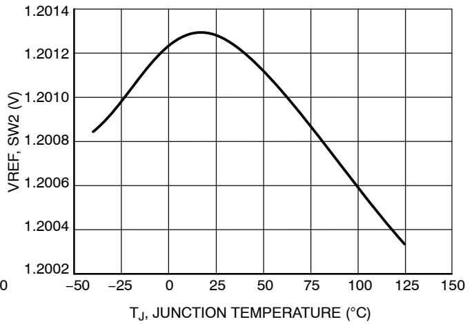
Figure 6. SW2 VREF vs. Junction Temperature
