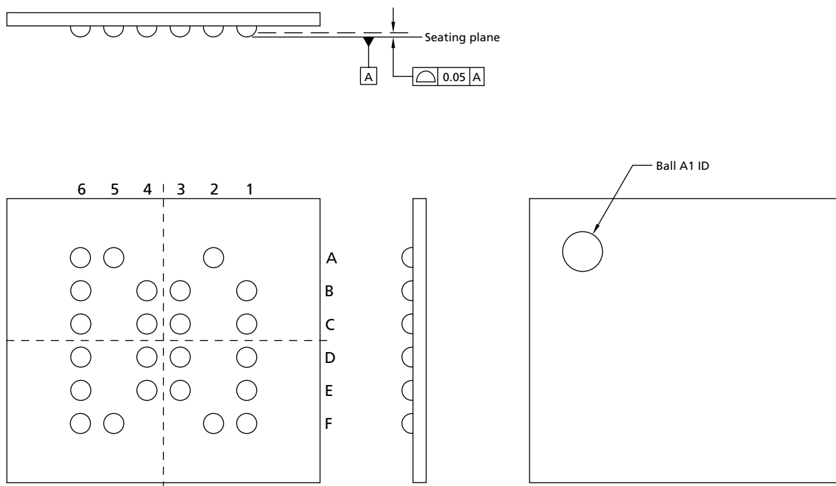
Figure 9: 23-Ball XFWLBGA
