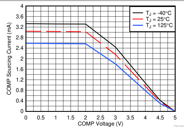
Figure 7-18. Error Amplifier Source Current
