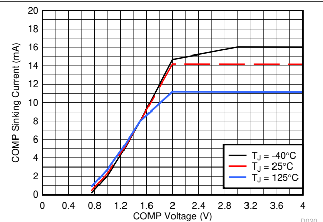
Figure 7-19. Error Amplifier Sink Current
