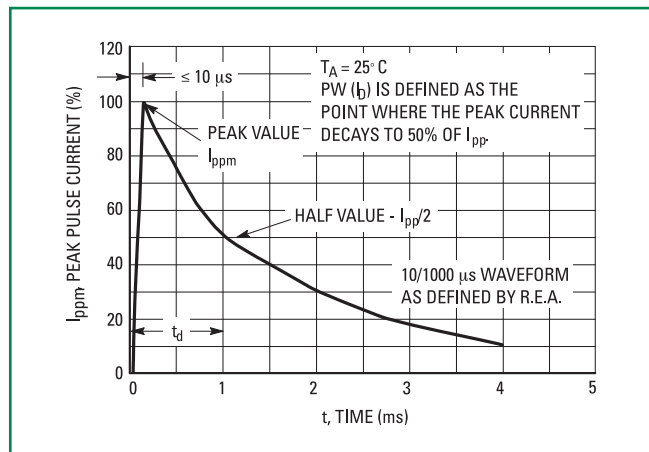
Figure 2. Pulse Waveform
