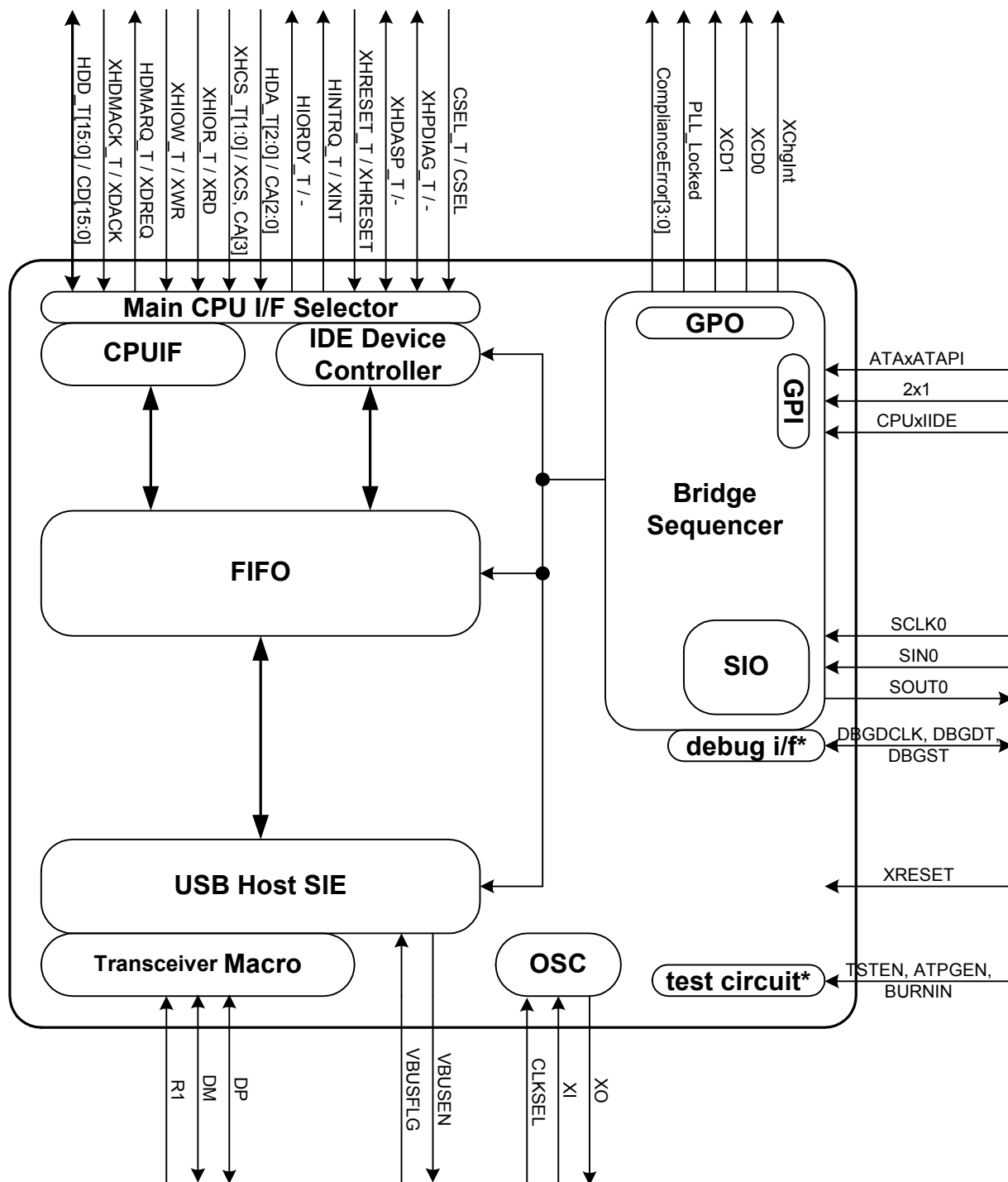
Figure 3.1 Block diagram
