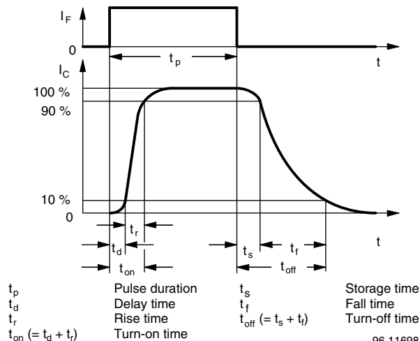
Fig. 2 - Switching Times
