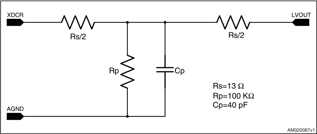
Figure 10. T/R SW signal equivalent circuit model
