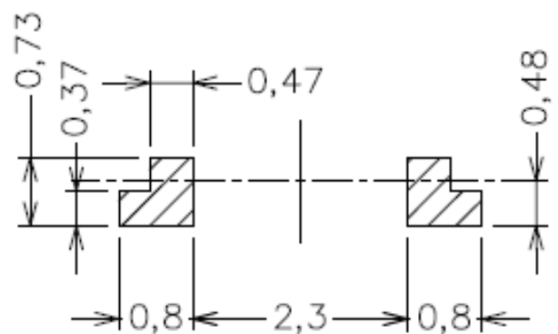
Soldering patterns
