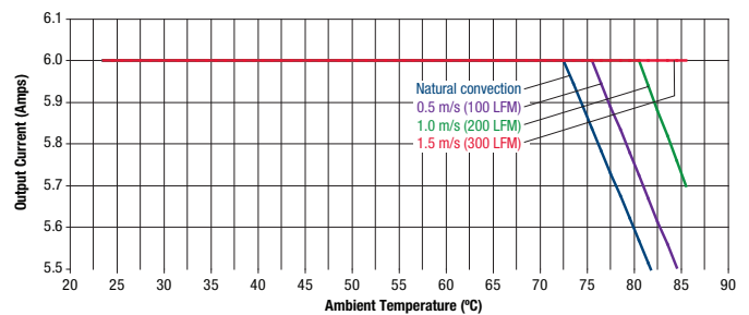
Maximum Current Temperature Derating @Sea Level (VIN = 18V, transverse airflow)
