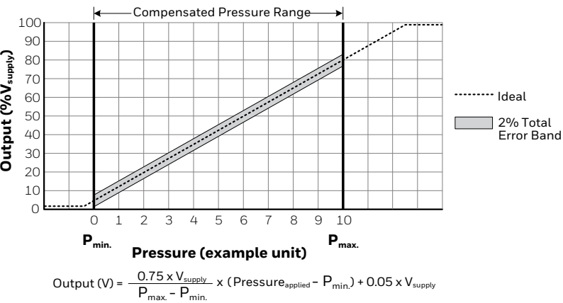
FIGURE 2. TRANSFER FUNCTION LIMITS
