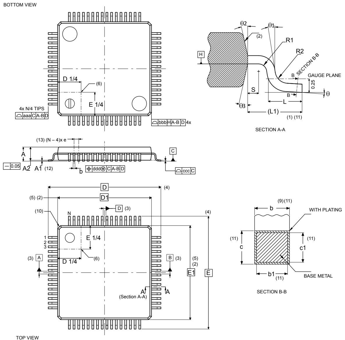
Figure 44. LQFP64 - Outline (15.)
