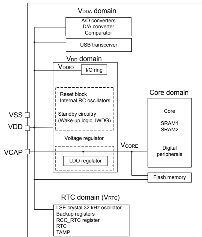
Figure 2. STM32C562xx power supply overview
