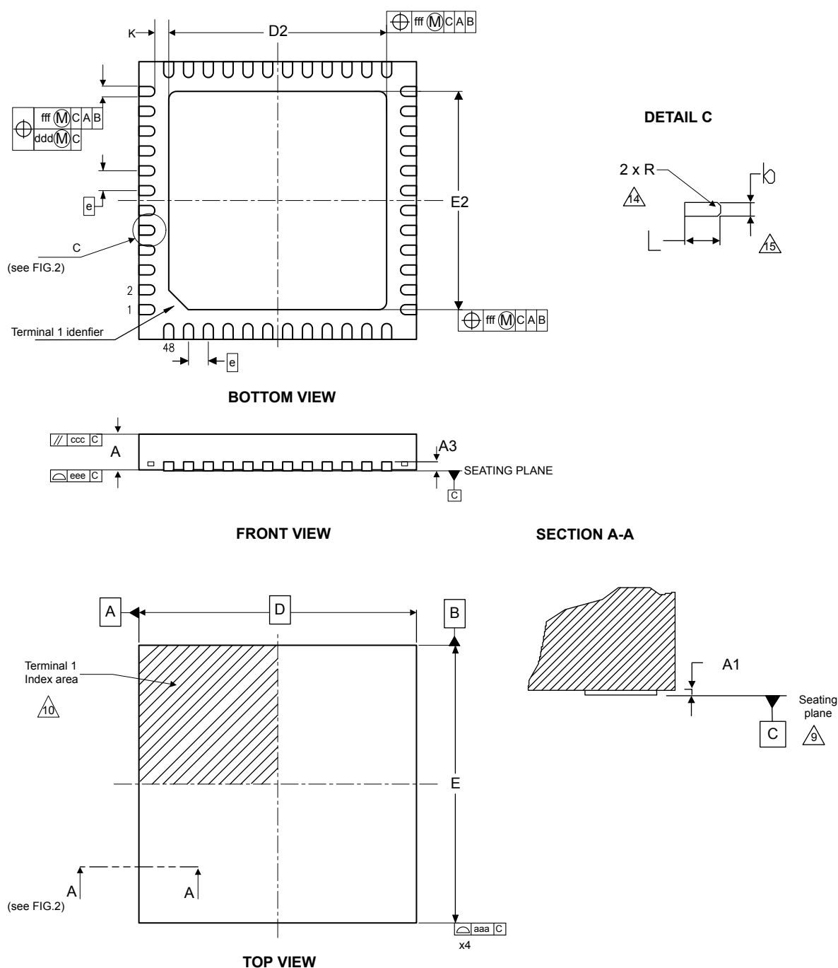
Figure 42. UFQFPN48 - Outline
