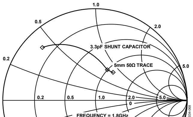
Figure 68. Effect of 50 \Omega PCB Trace on 50 \Omega Real Impedance Load
