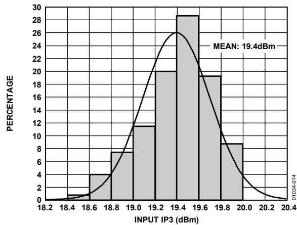
Figure 14. Input IP3 Histogram; f_{IN} = 900\text{ MHz} , f_{OUT} = 170\text{ MHz}
