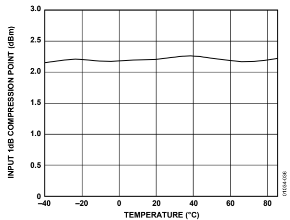
Figure 36. Input 1 dB Compression Point Performance Over Temperature; f_{IN} = 2400 \text{ MHz} , f_{OUT} = 425 \text{ MHz}
