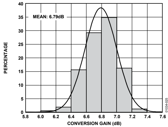
Figure 25. Gain Histogram; f_{IN} = 2400 \text{ MHz} , f_{OUT} = 170 \text{ MHz}
