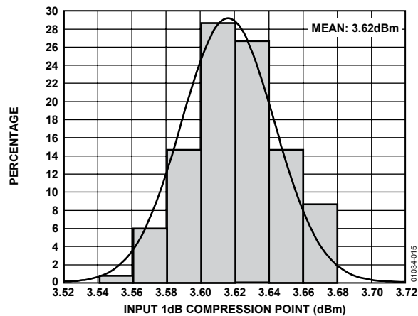
Figure 15. Input 1 dB Compression Point Histogram; f_{IN} = 900\text{ MHz} , f_{OUT} = 170\text{ MHz}
