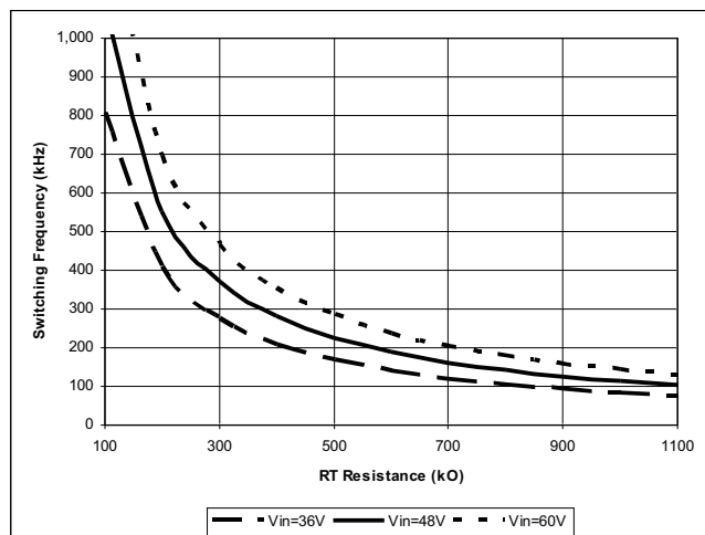
Figure 31. Nominal Switching Frequency of Converter vs Resistor RT
