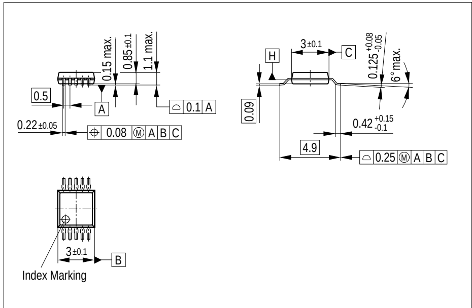
Figure 18 PG-TSSOP-10
