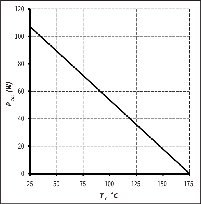
Figure 4. Power Derating
