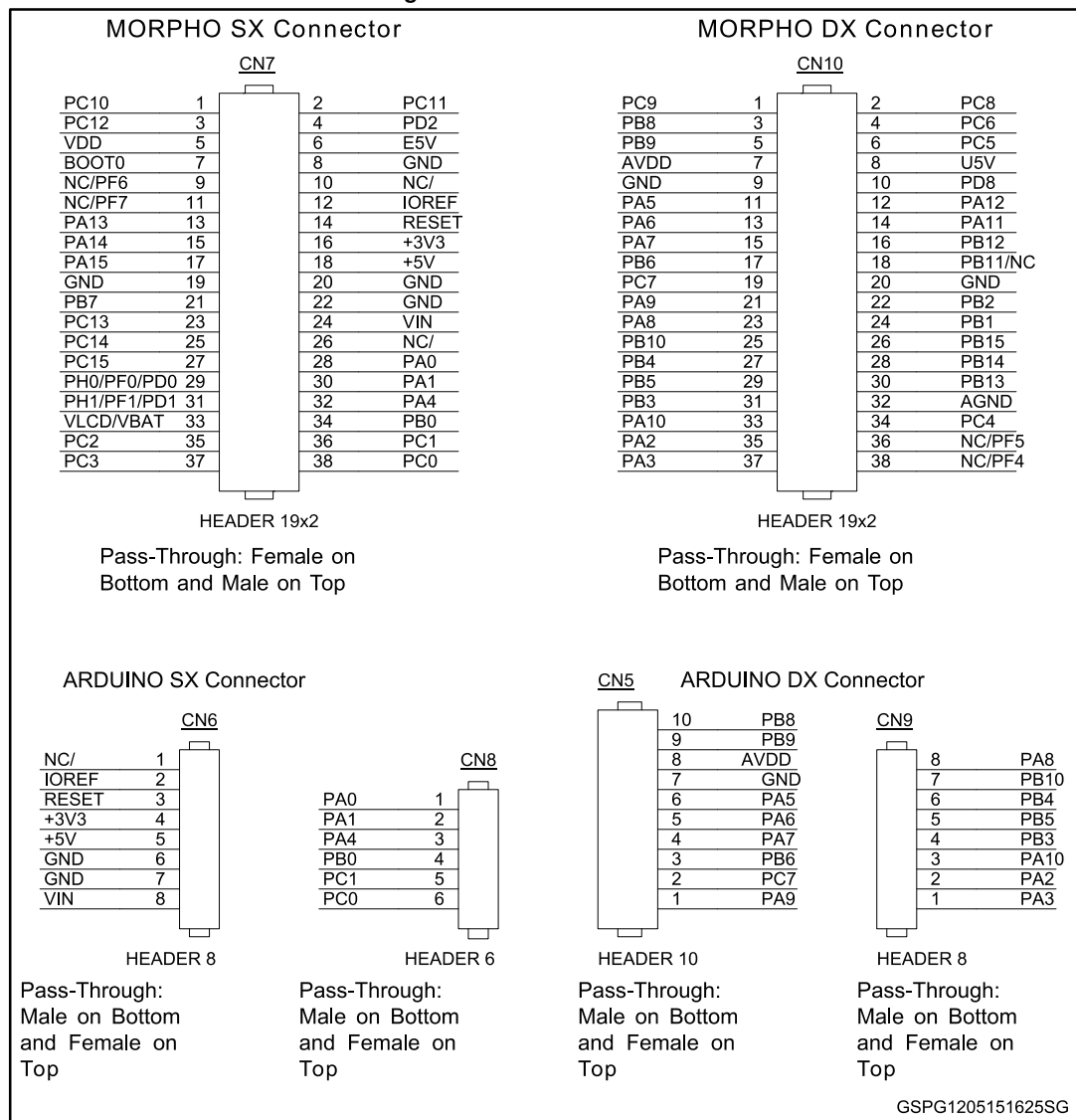
Figure 1: Nucleo connectors
