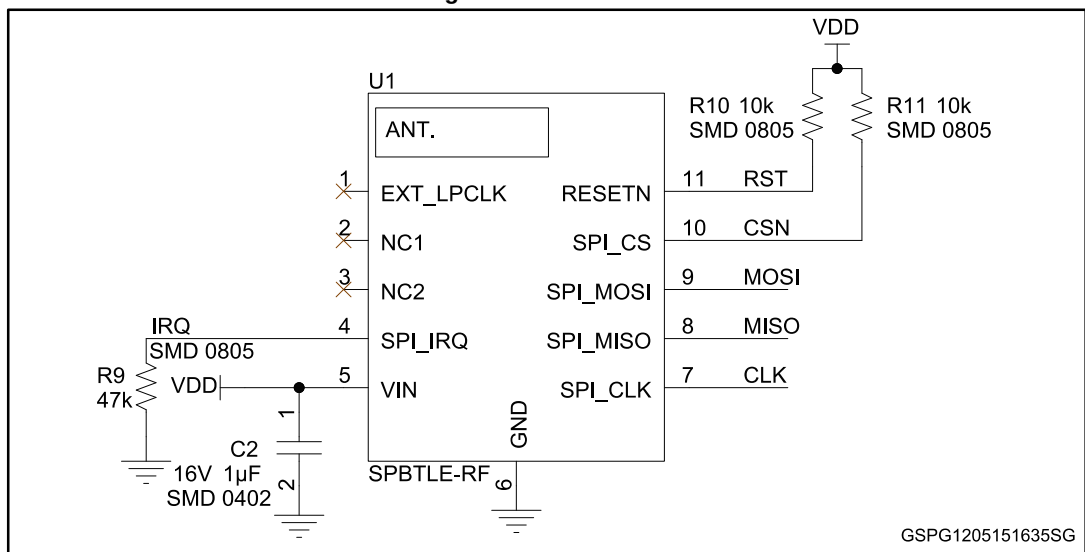
Figure 3: Nucleo connections
