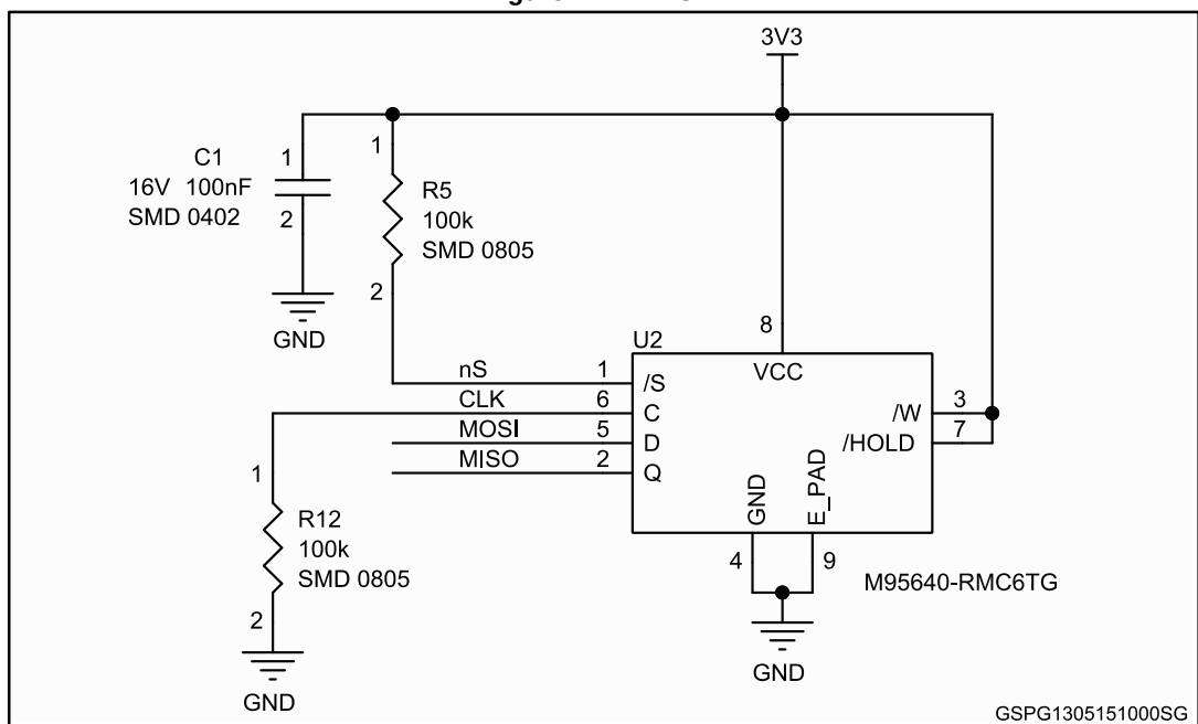
Figure 4: EEPROM
