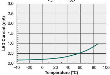
Typical I_F for Switch Dropout vs. Temperature ( I_L = 70\text{mA}_{\text{DC}} )
