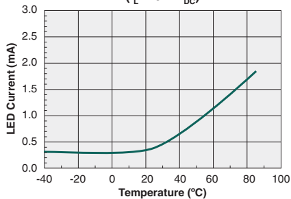
Typical I_F for Switch Operation vs. Temperature ( I_L = 70\text{mA}_{\text{DC}} )
