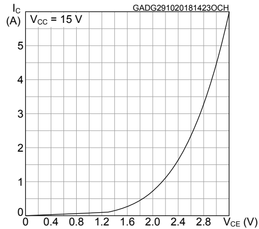
Figure 9. Output characteristics
