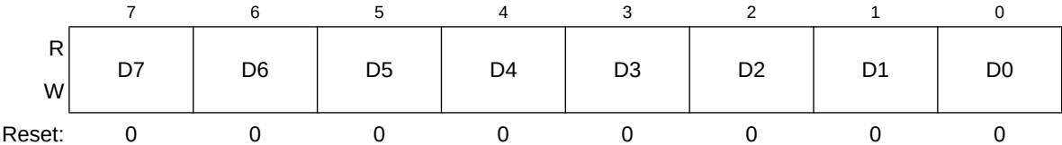
Figure 4-8. Linear Byte Post Increment Register (LBP)
