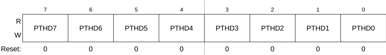
Figure 6-47. Port H Data Register (PTHD)
