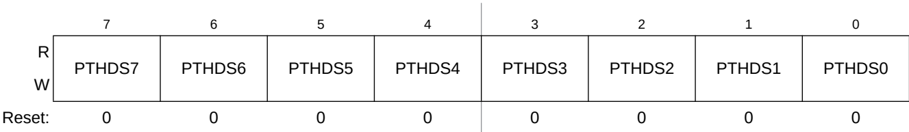
Figure 6-51. Drive Strength Selection for Port H Register (PTHDS)
