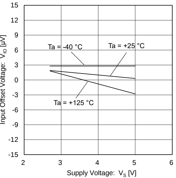
Figure 11. Input Offset Voltage vs Supply Voltage (V ICM = 0 V)
