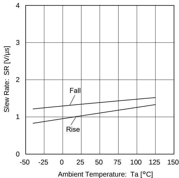
Figure 26. Slew Rate vs Ambient Temperature ( V_S = 2.7\text{ V} )
