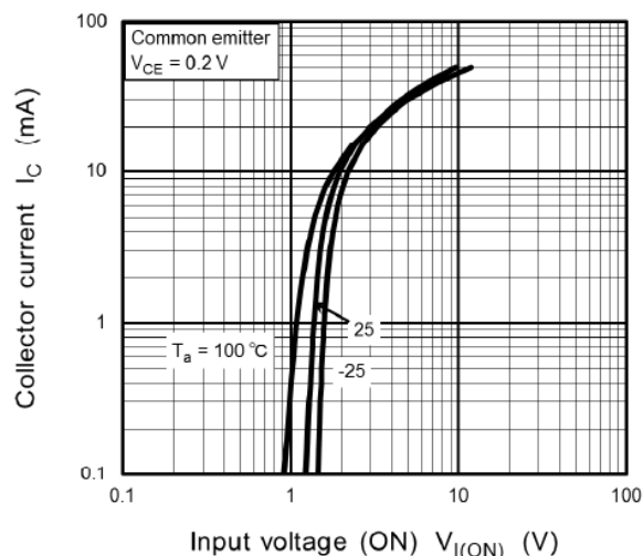
Fig. 11.1 RN1101MFV I_C - V_{I(ON)}
