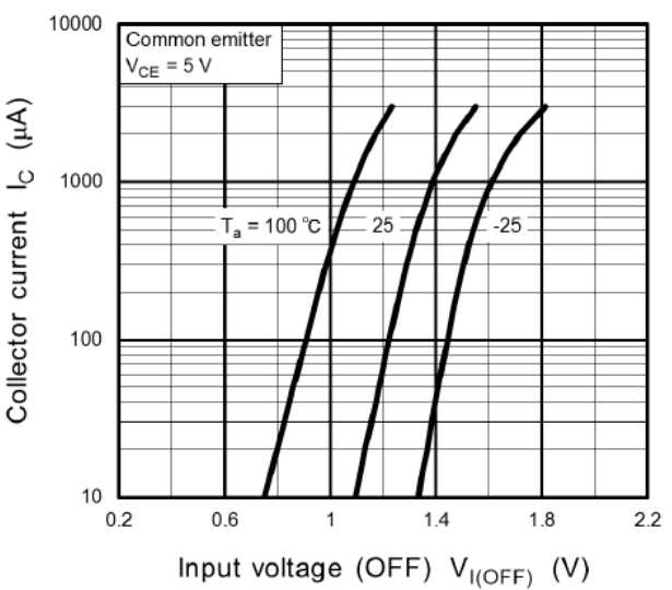
Fig. 11.8 RN1102MFV I_C - V_{I(OFF)}
