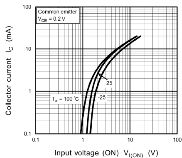
Fig. 11.4 RN1104MFV I_C - V_{I(ON)}
