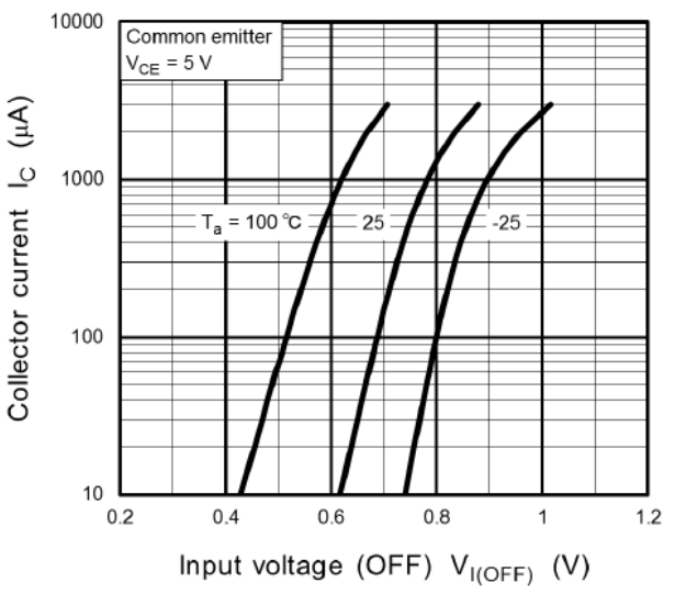
Fig. 11.12 RN1106MFV I_C - V_{I(OFF)}
