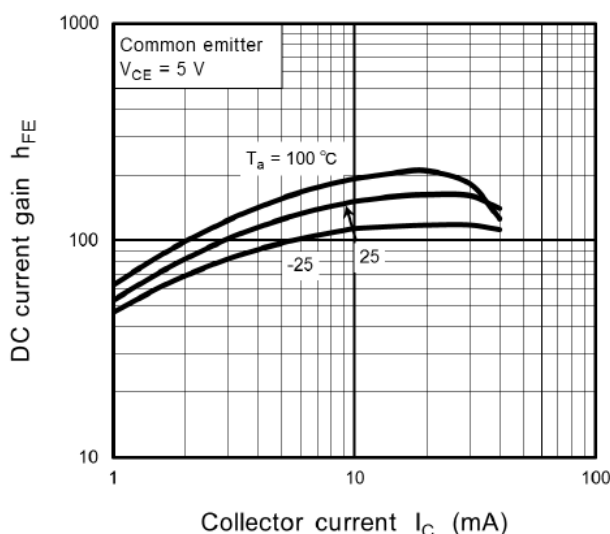
Fig. 11.16 RN1104MFV h_{FE} - I_C
