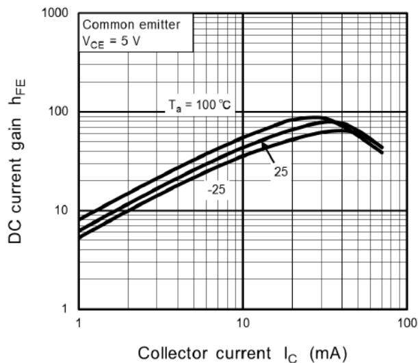
Fig. 11.13 RN1101MFV h_{FE} - I_C
