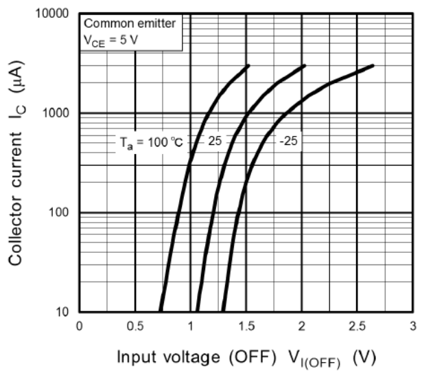
Fig. 11.10 RN1104MFV I_C - V_{I(OFF)}
