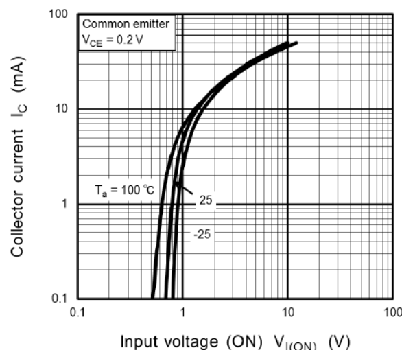
Fig. 11.6 RN1106MFV I_C - V_{I(ON)}
