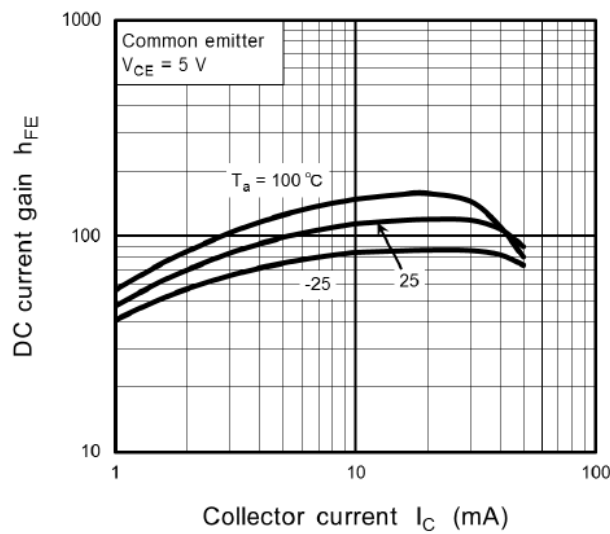
Fig. 11.18 RN1106MFV h_{FE} - I_C
