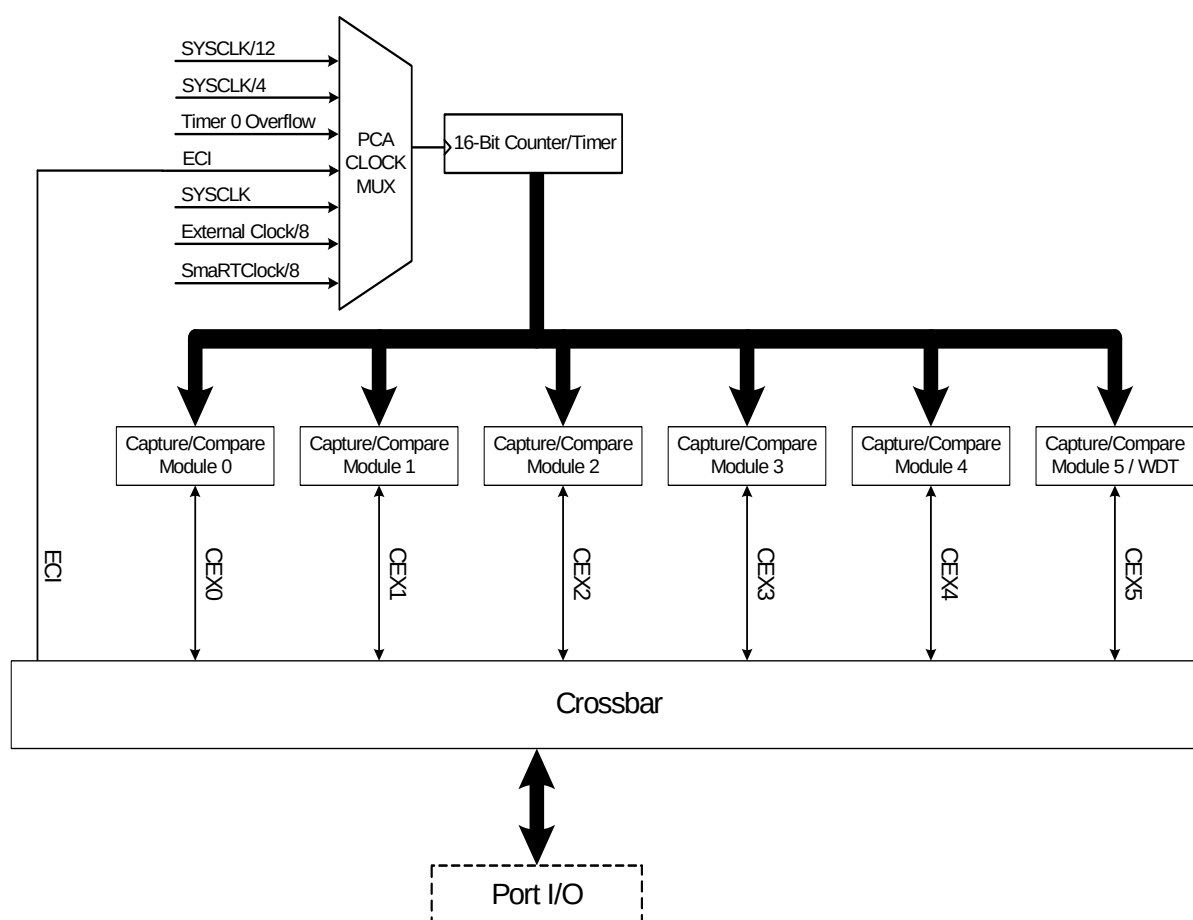
Figure 34.1. PCA Block Diagram
