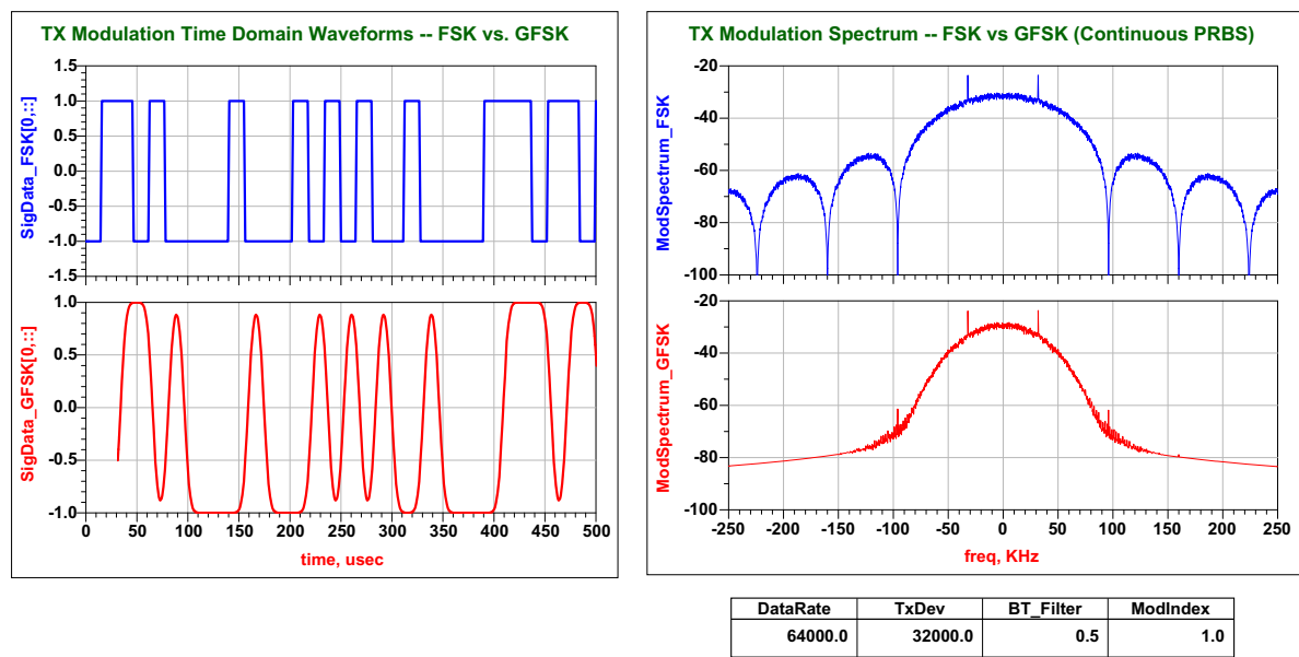
Figure 32.6. FSK vs. GFSK Spectrums
