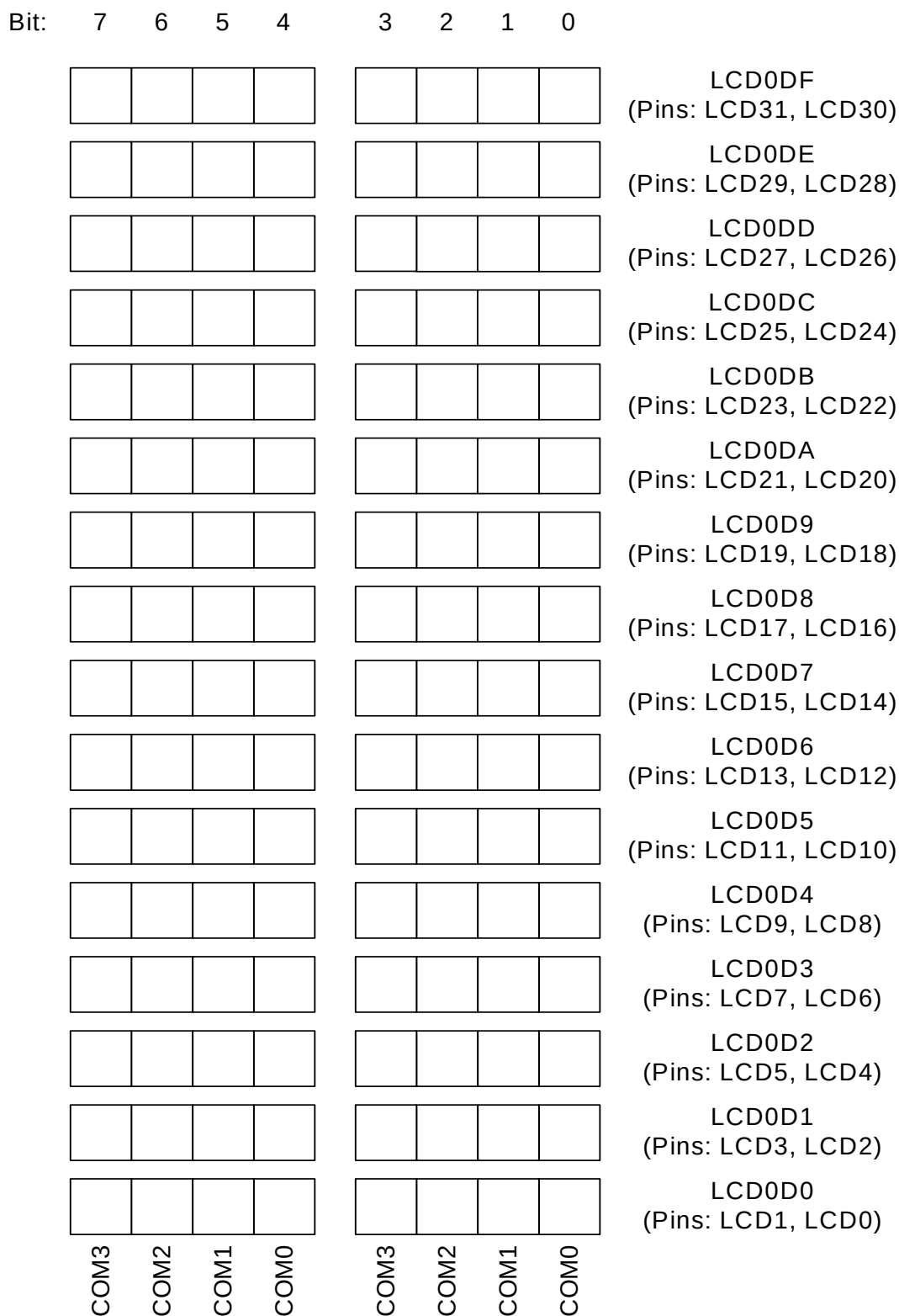
Figure 26.2. LCD Data Register to LCD Pin Mapping
