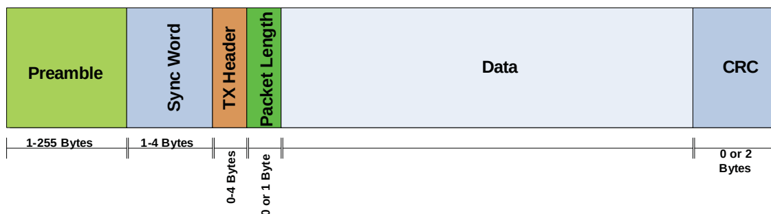
Figure 32.12. Packet Structure
