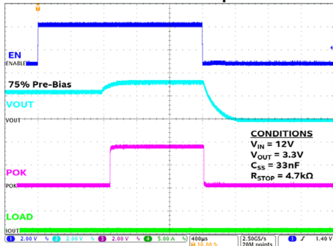
Pre-Bias Startup
