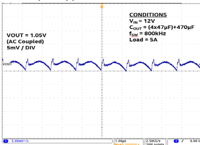
Output Ripple at 20MHz Bandwidth
