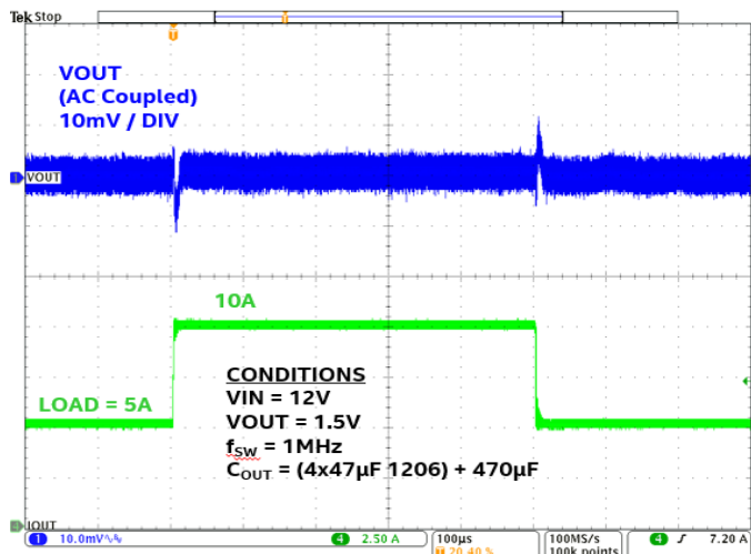
Load Transient 5 to 10A
