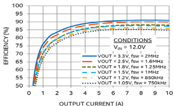
Figure 2: Efficiency at V_{IN} = 12 V
