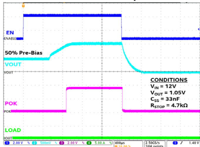
Pre-Bias Startup
