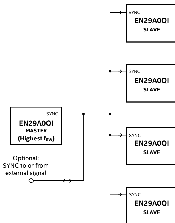
Figure 5: Frequency synchronization
