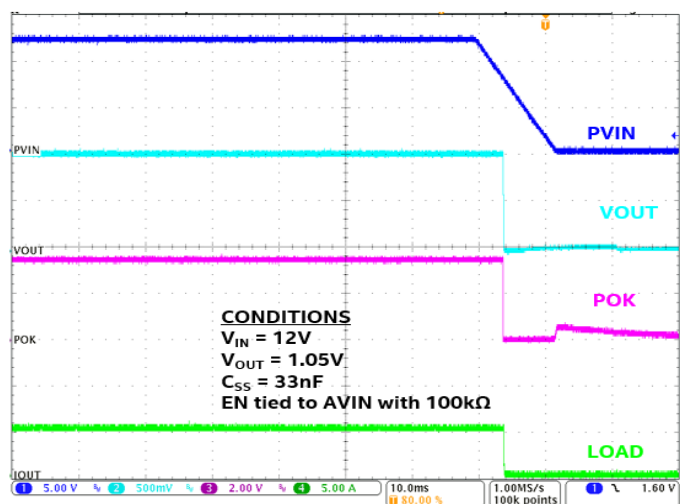
VIN Shutdown at 5A Load
