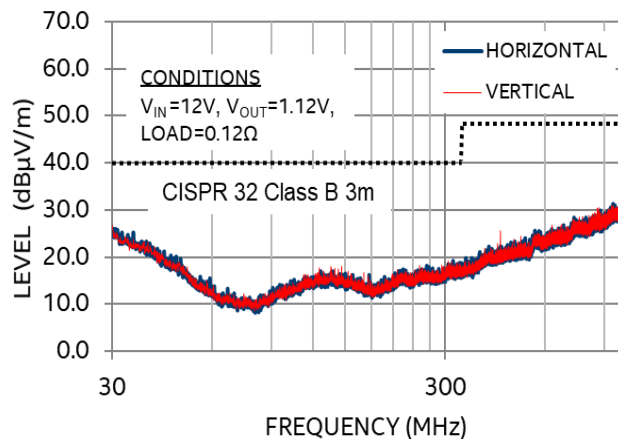
EMI Performance
