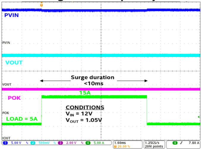
Surge current capability
