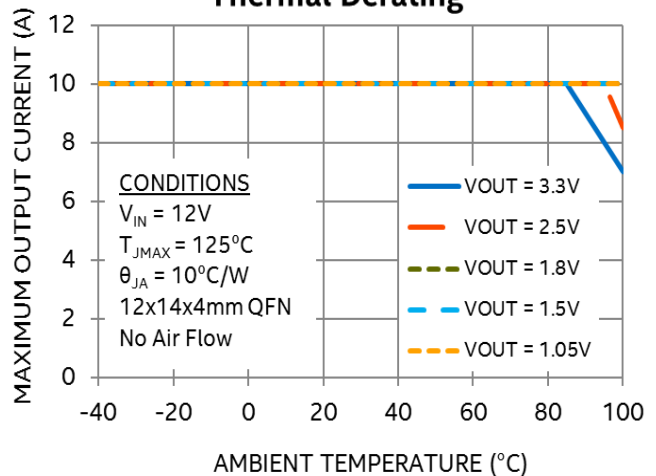
Thermal Derating
