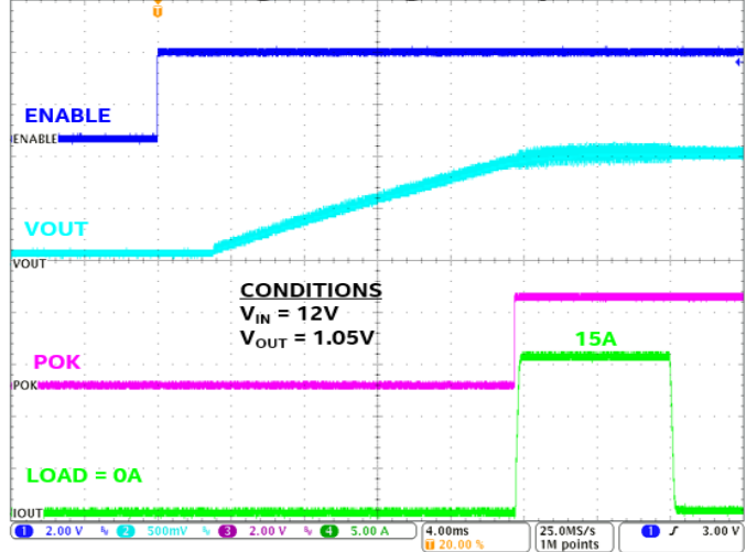
Surge during startup
