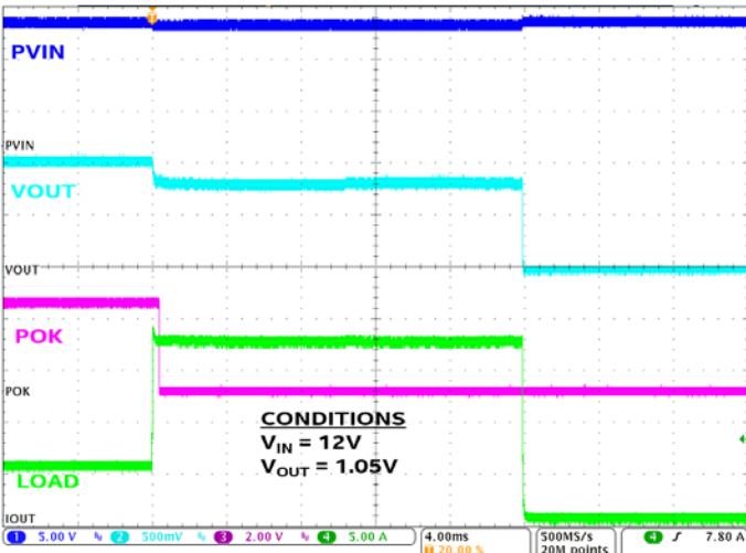
Short-circuit protection
