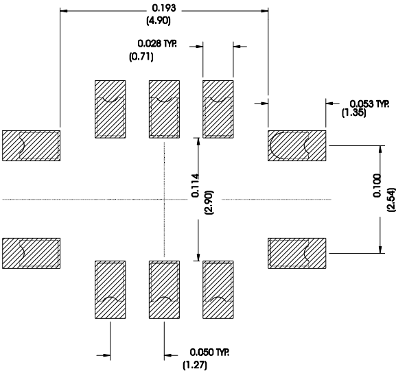
Recommended PCB Footprint
