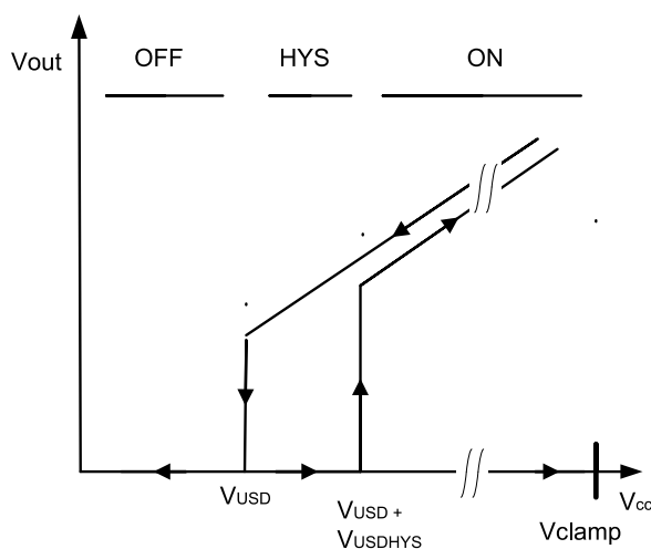
Figure 5. Undervoltage shutdown
