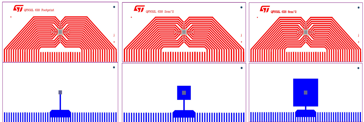
Figure 43. QFN 6x6 PCB 4 layers
