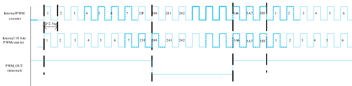
Figure 15. Resulting waveform 4
