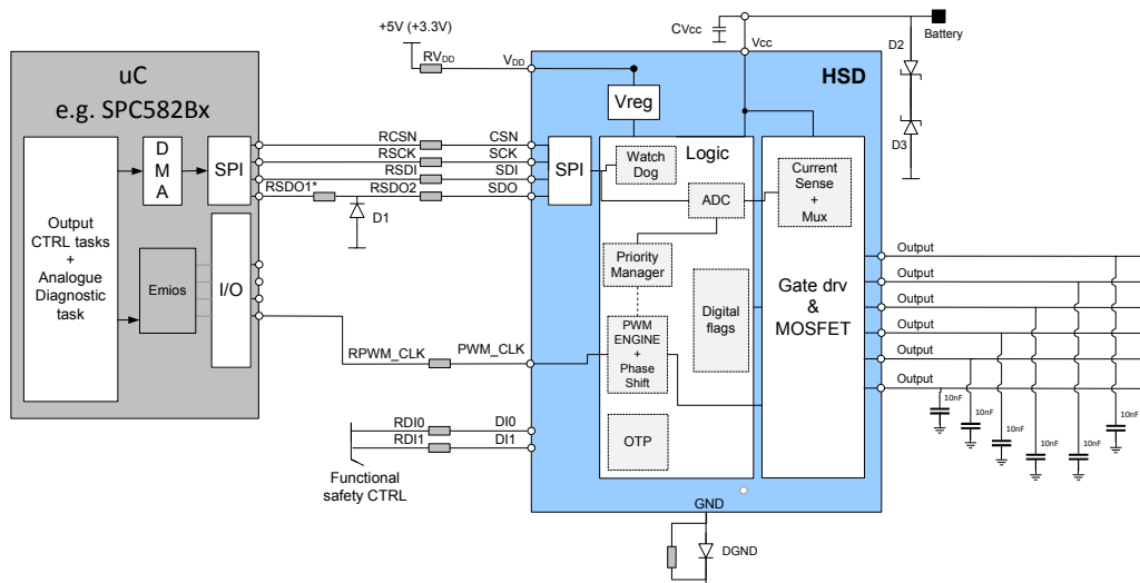
Figure 33. M0-9SPI application Schematic
