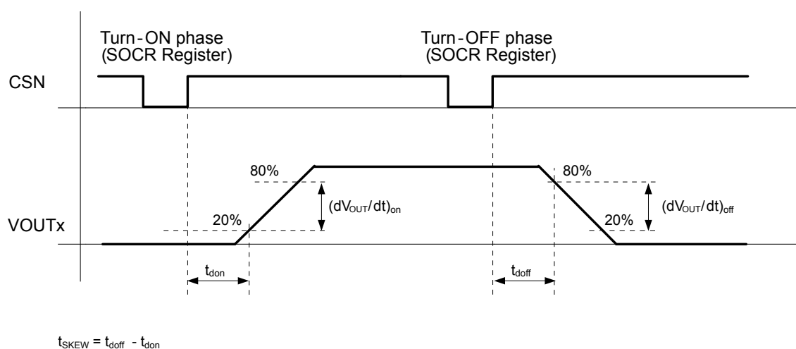
Figure 32. Switching characteristics
