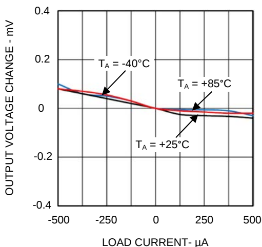
Load Regulation - \Delta V_{OUT}/\Delta I_{LOAD}
