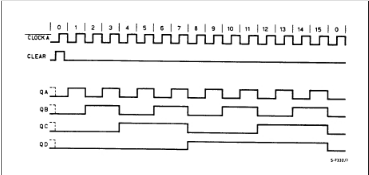
Figure 4: Timing Chart
