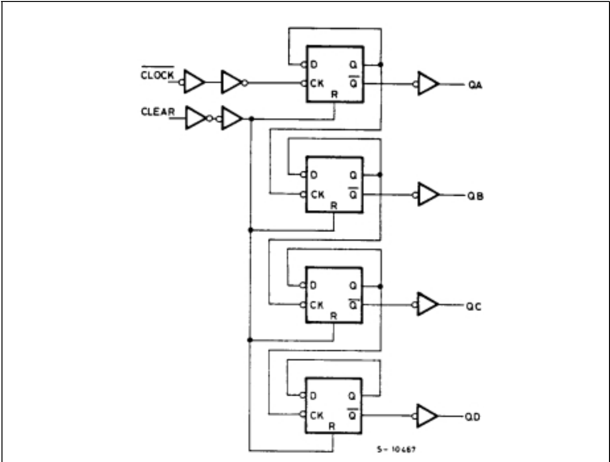
Figure 3: Logic Diagram
