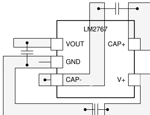
Figure 11-1. LM2767 Layout Example
