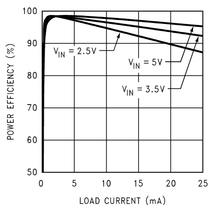
Figure 9-6. Efficiency vs Load Current
