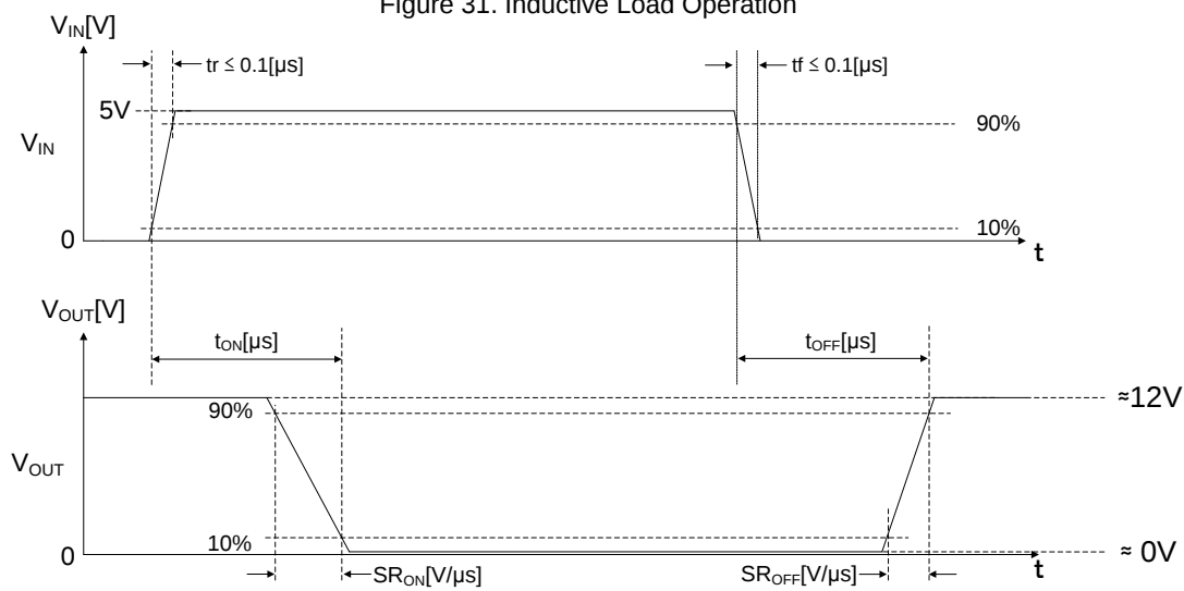
Figure 32. Switching Time
