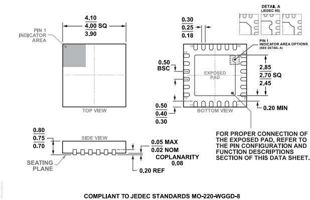
Figure 36. 24-Lead Lead Frame Chip Scale Package [LFCSP] 4 mm × 4 mm Body and 0.75 mm Package Height (CP-24-8) Dimensions shown in millimeters
