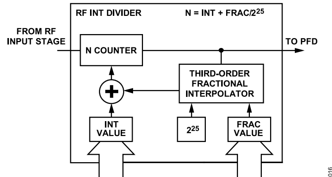
Figure 14. Fixed Modulus N Divider
