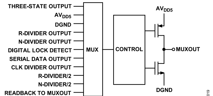
Figure 17. MUXOUT Schematic
