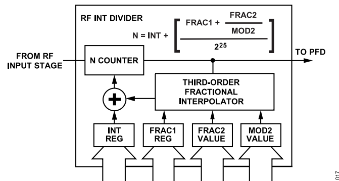
Figure 15. Variable Modulus N Divider
