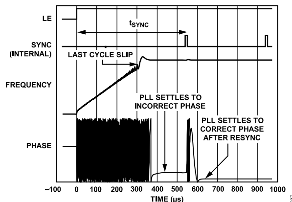
Figure 35. Phase Resync Example
