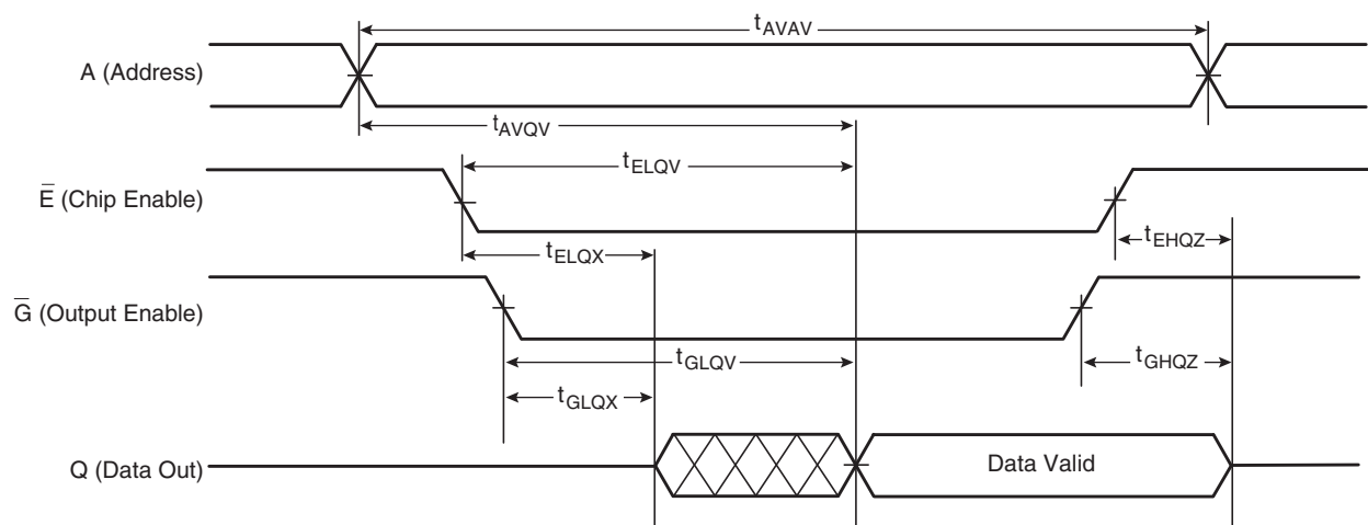
Figure 3-4. Read Cycle 2
