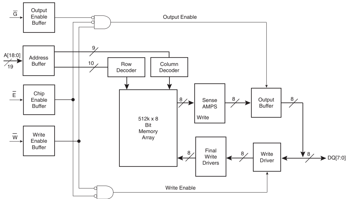
Figure 1-1. Block Diagram
