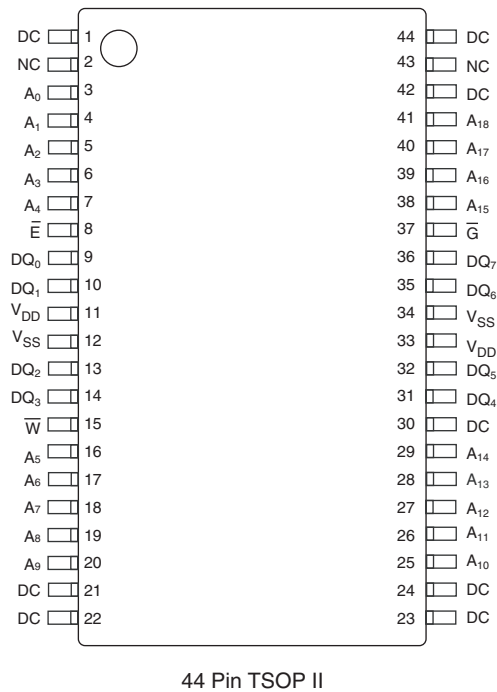
Figure 1-2. Pin Diagrams for Available Packages (Top View)
