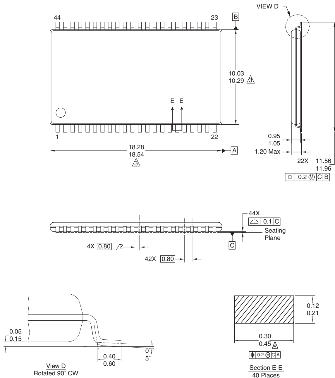
Figure 4-1. TSOP2
