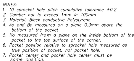
Figure 24: Carrier Tape Dimensions
