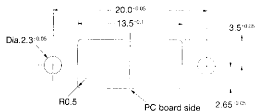
Panel Cutout
