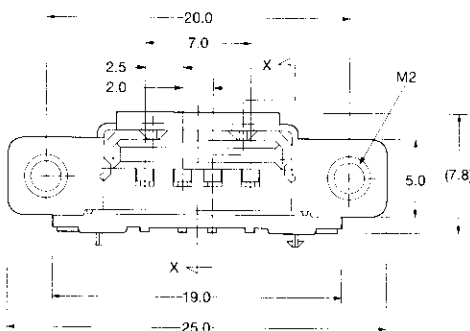
Tape (#353929-1 only)
