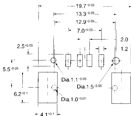
PC Board Layout (Component Side)
