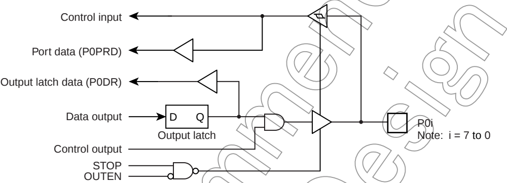
Figure 5-2 Port 0
