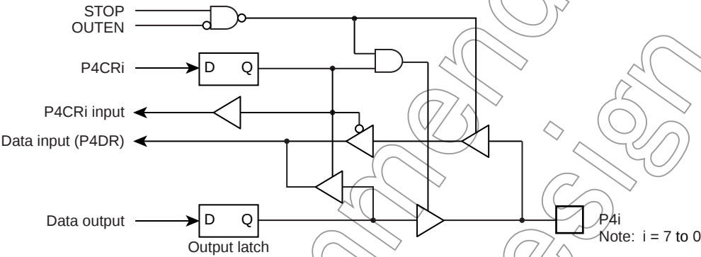
Figure 5-6 Port P4
