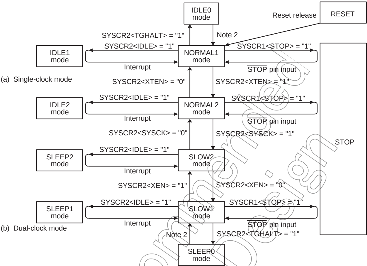
Figure 2-6 Operating Mode Transition Diagram
