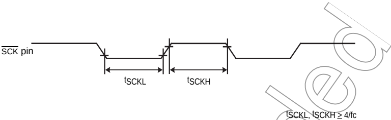
Figure 10-3 External Clock
