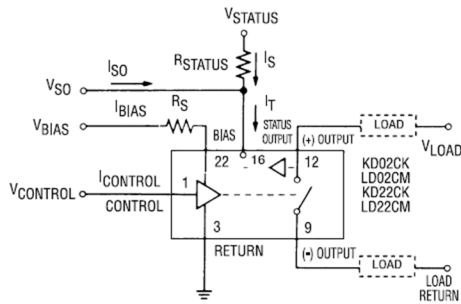
(A) 3 Terminal Input with Status (See Note 5)
