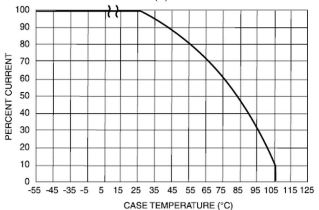
LOAD CURRENT DERATING CURVE FOR LD SERIES WITH HEAT SINK (B)
