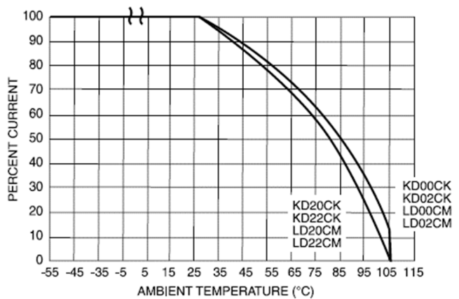
LOAD CURRENT DERATING CURVE FOR KD/LD SERIES WITHOUT A HEAT SINK (A)
