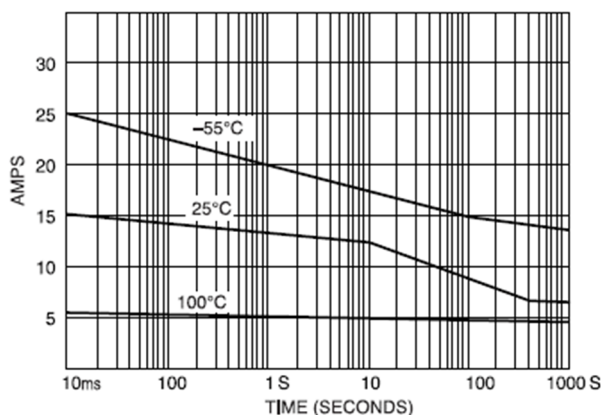
OVERLOAD CURRENT VS TIME TO TRIP (TYPICAL) KD20CK, KD22CK, LD20CM, LD22CM FIGURE 7
