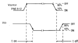
STATUS TURN-ON AND TURN-OFF TIMING FIGURE 6
