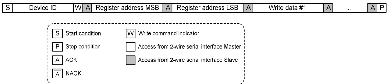
Figure 5. 2-wire serial I/F write to THCV242A local register protocol
