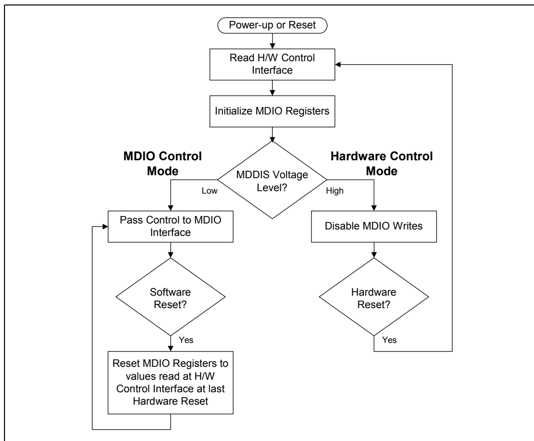
Figure 13 Initialization Sequence
