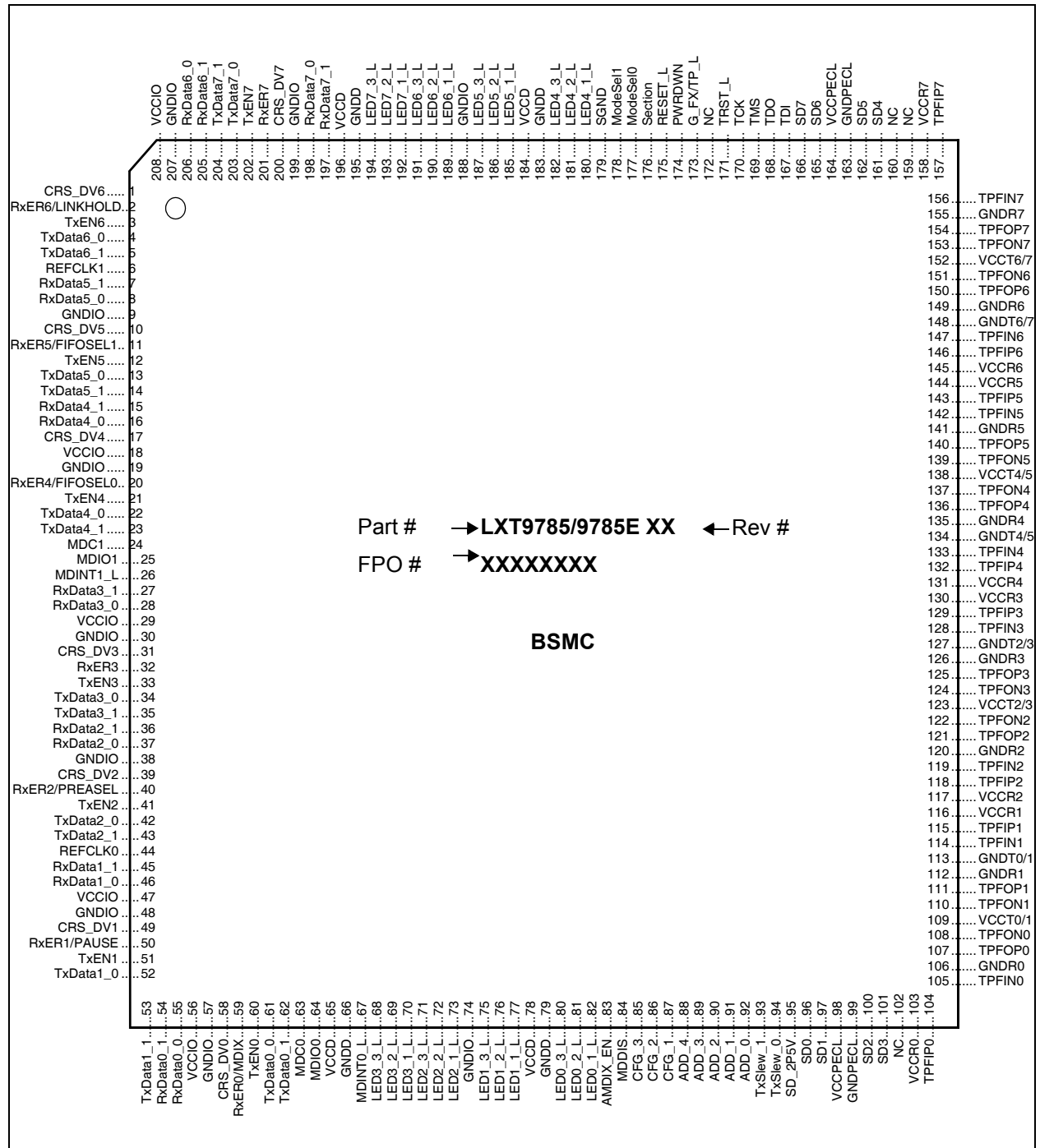
Figure 2 RMII 208-Pin PQFP Assignments
