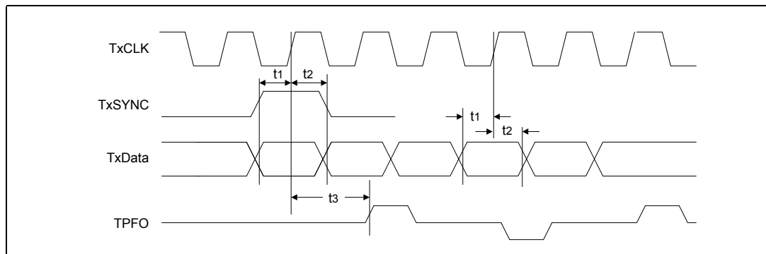
Figure 48 SS-SMII - 100BASE-FX Transmit Timing
