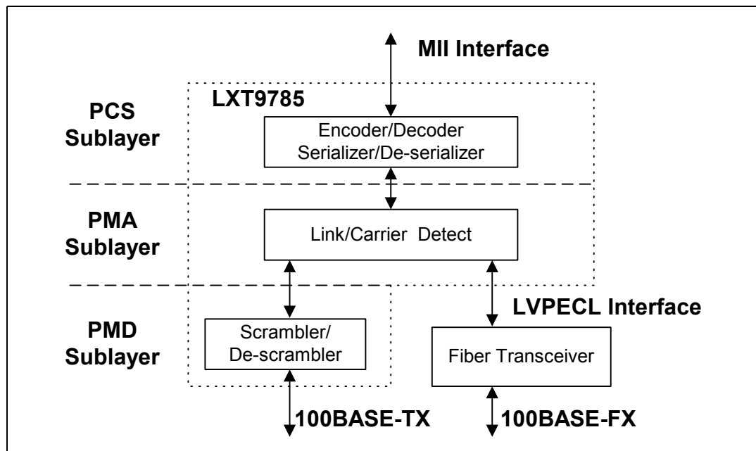
Figure 28 Protocol Sublayers
