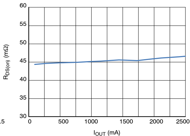
Figure 5. R_{DS(on)} (mΩ) vs. I_{load} (mA) at 3.6 V
