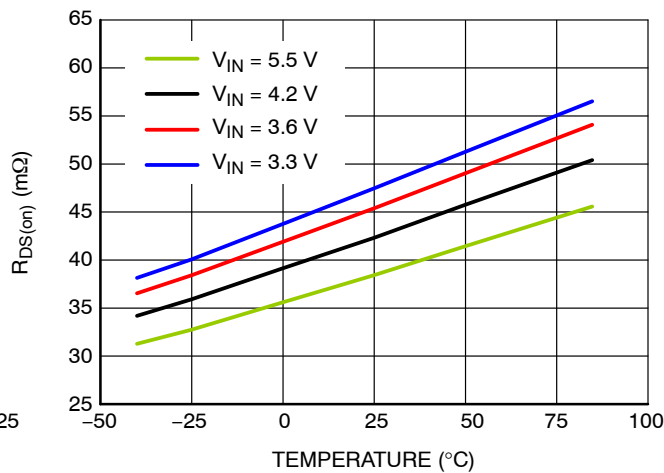
Figure 7. R_{DS(on)} (mΩ) vs. Temperature (°C), I_{load} 2 A
