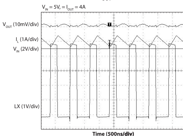
Output Voltage Ripple ( V_{OUT}=1.5\text{V} ) @ Full Load
