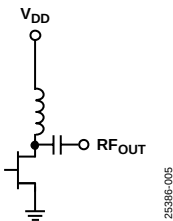
Figure 6. V DD and RF OUT Interface Schematic
