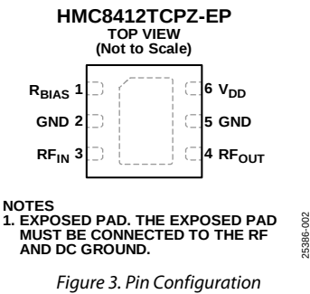
Figure 3. Pin Configuration
